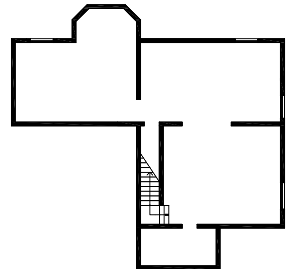
Basement plan
