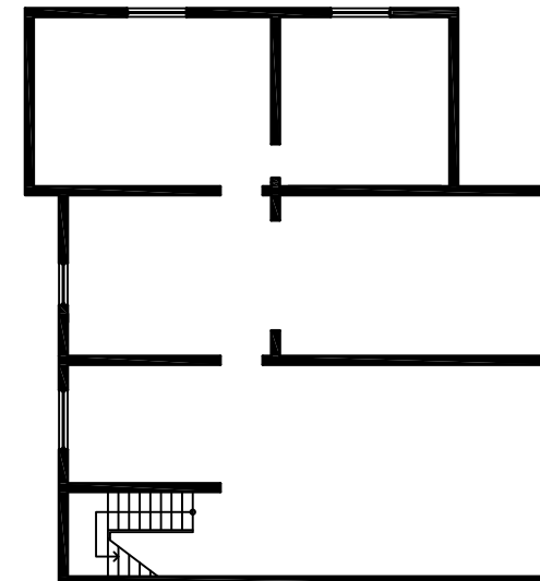
Basement plan
